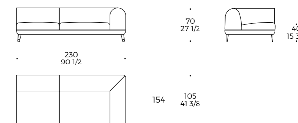
Elemento 3 posti grande Br Dx 3 seater element maxi Arm R Élément 3 places maxi Br D
