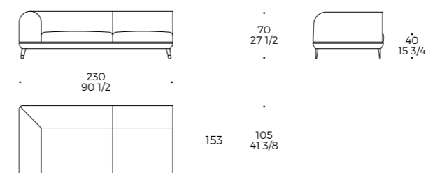
Elemento 3 posti grande Br Sx 3 seater element maxi Arm L Élément 3 places maxi Br G
