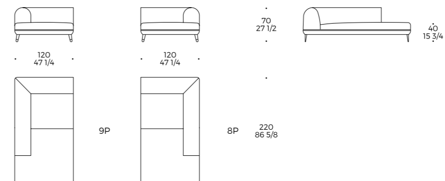
Elemento terminale piccolo Br Sx (9P) / Dx (8P) Small terminal element L (9P) / R (8P) Arm Élément petit terminal Br C (9P) / D (8P)
